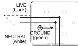
FIXTURE CABLES
