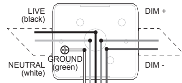
FIXTURE CABLES
