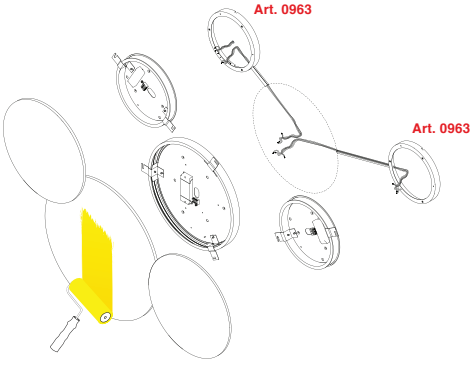
Example of multiple installation with spacers.
