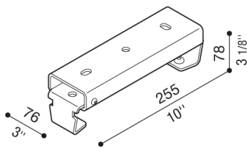
Ceiling bracket
