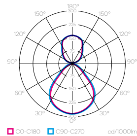
light distribution UP & DOWN
