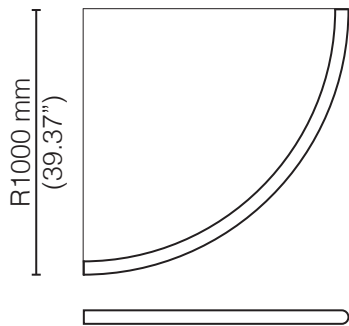
FREEDOM LINE+ R100-90° L56LINER10090D
