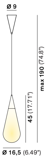
Goccia H2 Light source: E26 LED 8W
