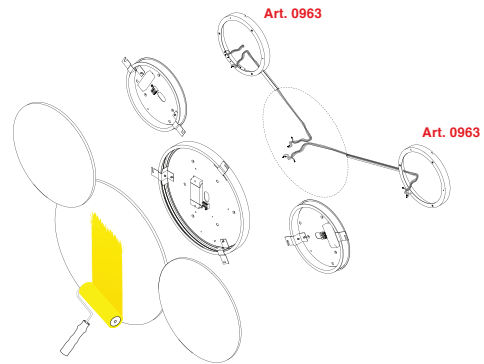
Example of multiple installation with spacers.
