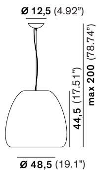
L16POMIH1 Light source: E26 LED max watt 15W
