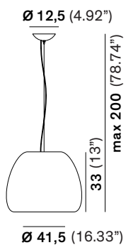
Pomi L16H2 Light source: E26 LED max watt 15W
