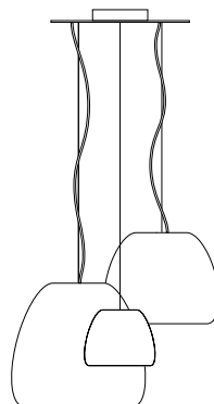
Composition example with optional ø50 (ø19.65") canopy. Maximum 6 lights. Order code: R1.
