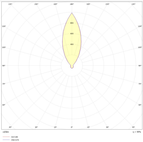
Photometric curves
