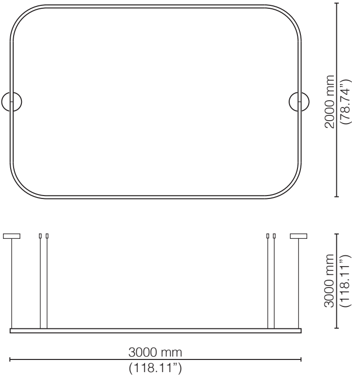
BIG-O RECTANGLE 3000 x 2000
