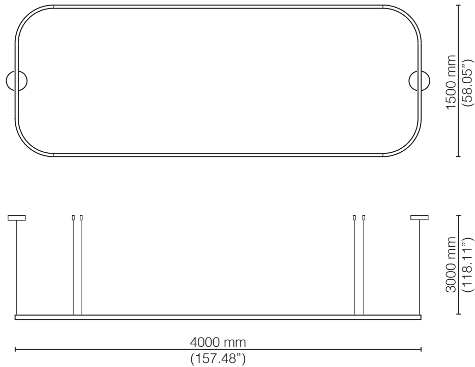
BIG-O RECTANGLE 4000 x 1500
