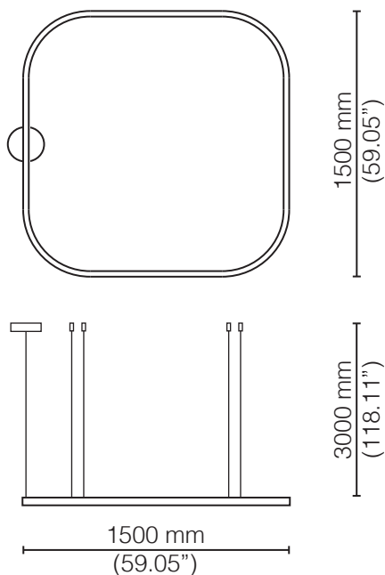
BIG-O SQUARE 1500 x 1500
