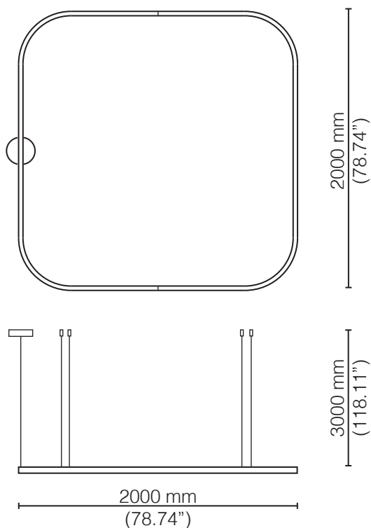
BIG-O SQUARE 2000 x 2000
